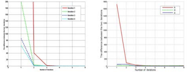
Figure 2. Convergence of the proposed coding algorithm (left) and the proposed joint discriminative dictionary, sparse codes and classifier learning algorithm (right).
