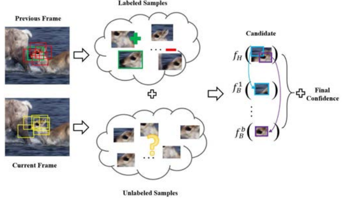
Figure 1. Confidence calculation. The holistic classifier f_H and block classifiers f_B^1, \dots, f_B^b are trained with labeled and unlabeled samples. Given a candidate, classifiers are applied to classify their corresponding blocks. The final confidence of a candidate is a weighted sum of holistic and block classifiers.
