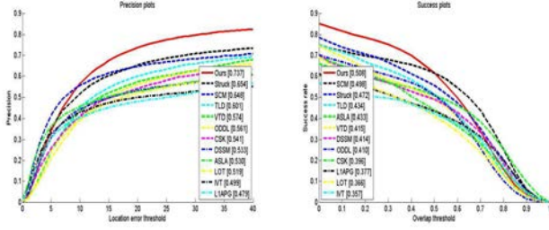
Figure 3. Overall performance comparisons of precision plot (left side) and success rate (right side) for these trackers. The overall performance score at 20 pixel is presented in the legend.
