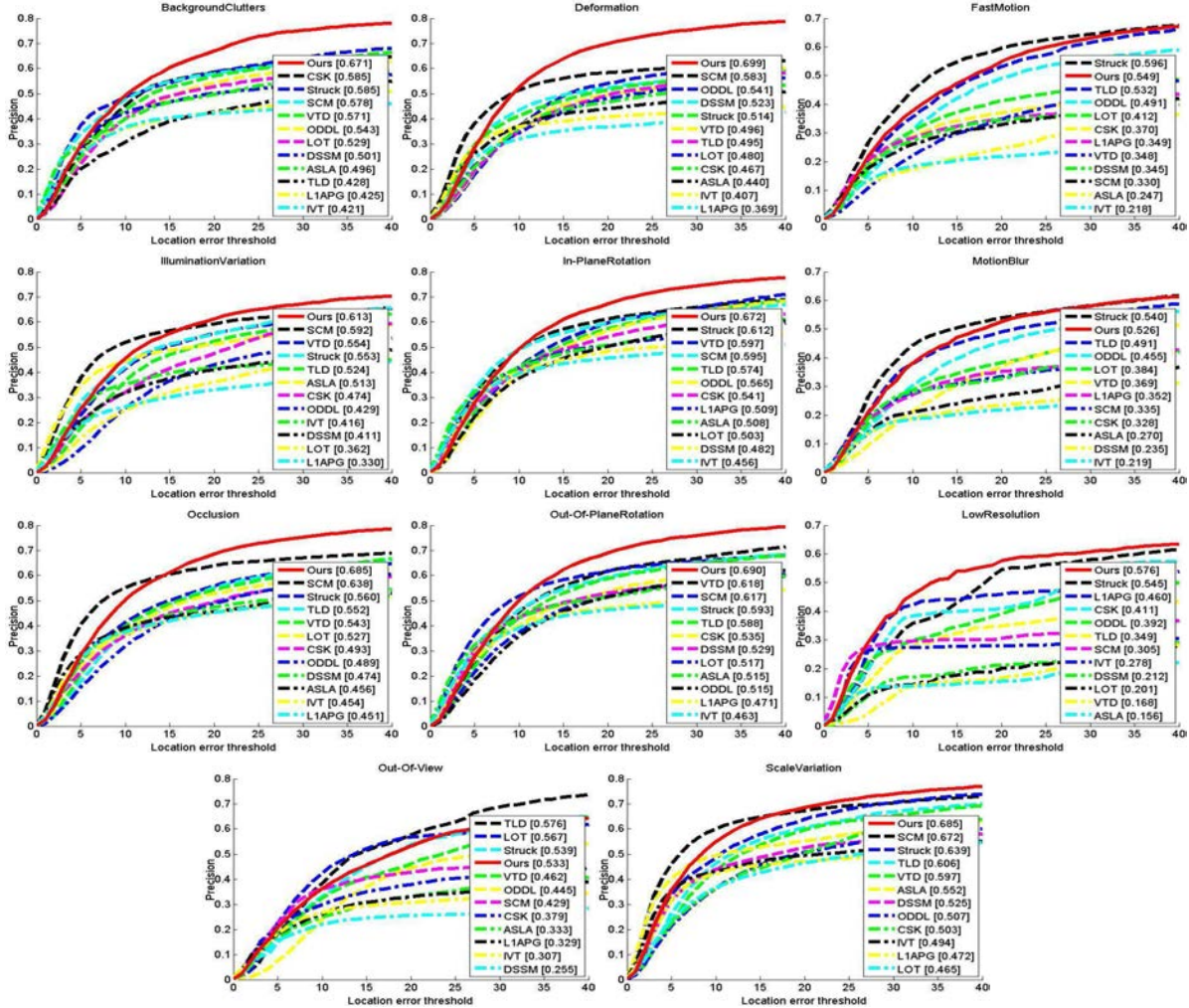
Figure 4. Attribute-based estimation comparisons of precision plots for these trackers.
